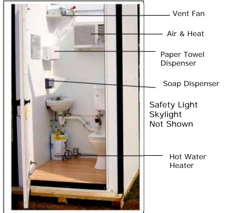
Fig. 5 Front View Open Door
